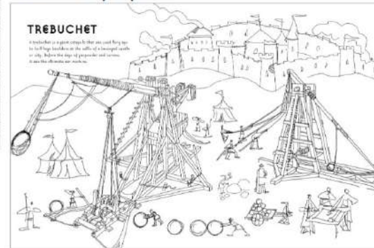
Trebuchet sample spread
