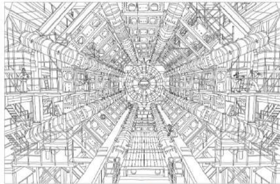
Hadron collider sample spread
